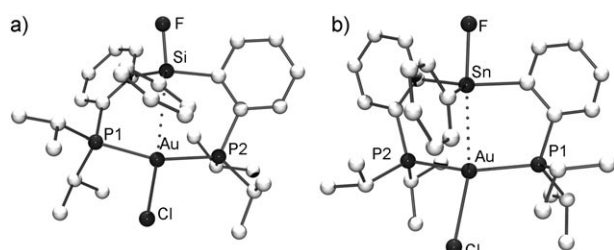
Figure 1. Molecular views of complexes 2 (a) and 4 (b) in the solid state (hydrogen atoms omitted for clarity). Selected bond lengths [Å] and angles [°]: 2 : P1–Au 2.323(2), P2–Au 2.305(2), Au–Cl 2.577(2), Si–F 1.635(3), Au–Si 3.090(2); P1–Au–P2 140.14(5), Cl–Au–Si 141.54(4), Au–Si–F 166.11(12). 4 : P1–Au 2.334(2), P2–Au 2.330(2), Au–Cl 2.601(2), Sn–F 2.018(3), Au–Sn 2.891(2); P1–Au–P2 159.91(6), Cl–Au–Sn 151.36(4), Au–Sn–F 176.27(9).
